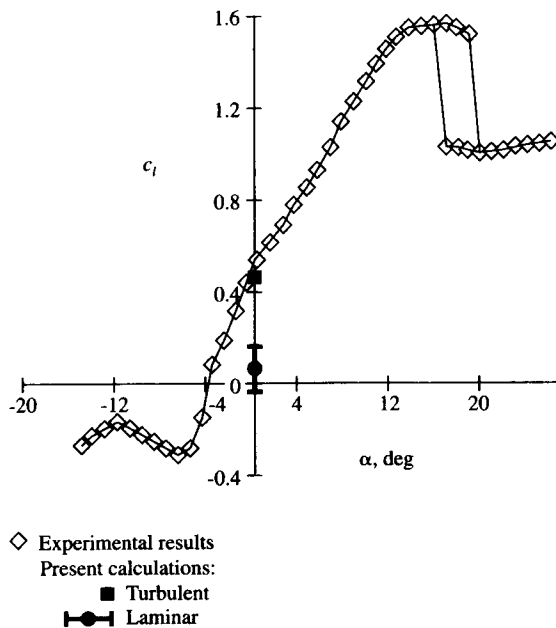
FIG. 1.4 Example of a CFD numerical experiment. Lift coefficient versus angle of attack for a Wortmann airfoil. Re = 100,000 ; M_\infty = 0.5 .
