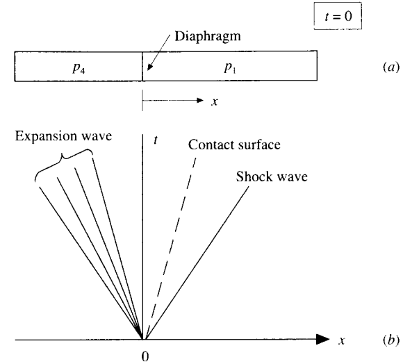
FIG. 11.6 Wave diagram.
