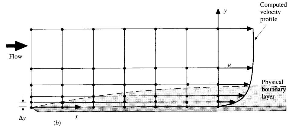
FIG. 5.11 Two sketches demonstrating the need to concentrate a number of grid points in the boundary layer. (a) No grid points in the boundary layer; (b) at least some points in the boundary layer.
