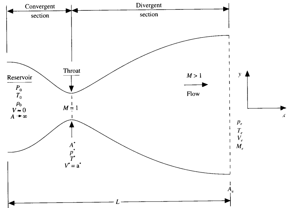
FIG. 7.1 Schematic for subsonic-supersonic isentropic nozzle flow.
