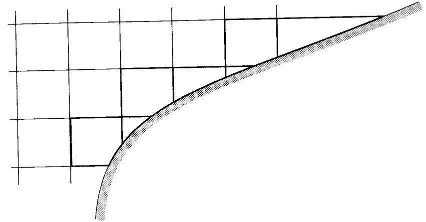
FIG. 5.18 Section of a cartesian mesh near a surface. Those mesh cells adjacent to the surface are highlighted by bold lines; they are modified so that one side of the cell lies along the surface.
