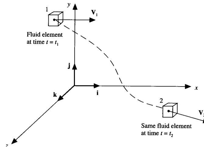
FIG. 2.3 Fluid element moving in the fluid flow—illustration for the substantial derivative
