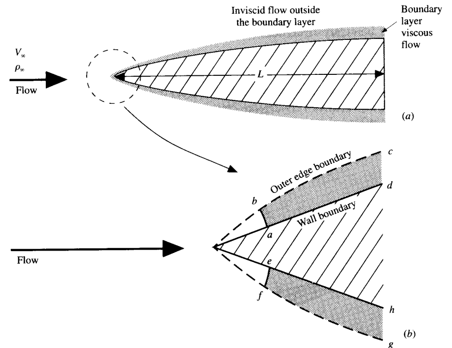
FIG. 3.10 Schematic of a boundary-layer flow.
