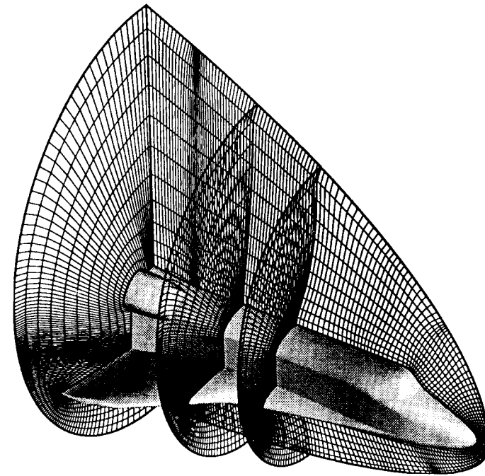
FIG. 6.32 A three-dimensional mesh plot for the calculation of the flow over a body, where the body is shown as a light-source-shaded surface. (From Ref. 72. Courtesy of Amtec Engineering, Bellevue, Washington.)
