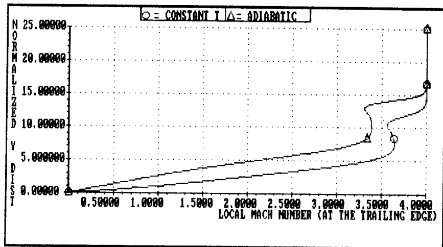
FIG. 10.15 Mach 4 at sea level: local Mach number profiles at the trailing edge.
