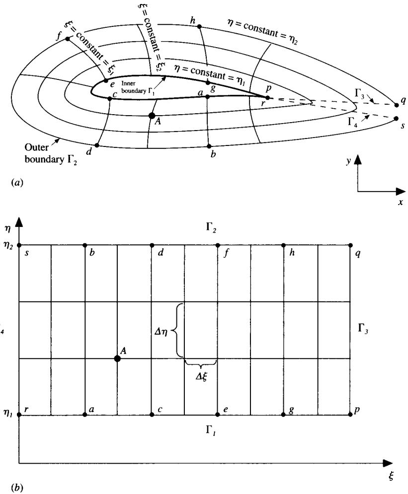
FIG. 5.7 Schematic of an elliptically generated, boundary-fitted grid. (a) Physical plane; (b) computational plane.
