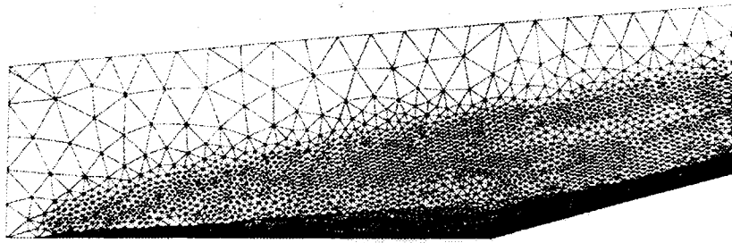
FIG. 5.17 An unstructured mesh around a compression corner. (From Ref. 40. Copyright © 1991, AIAA. Reprinted with permission.)
