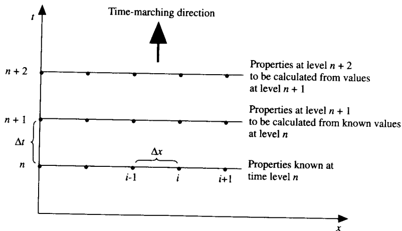
FIG. 4.6 Illustration of time marching.
