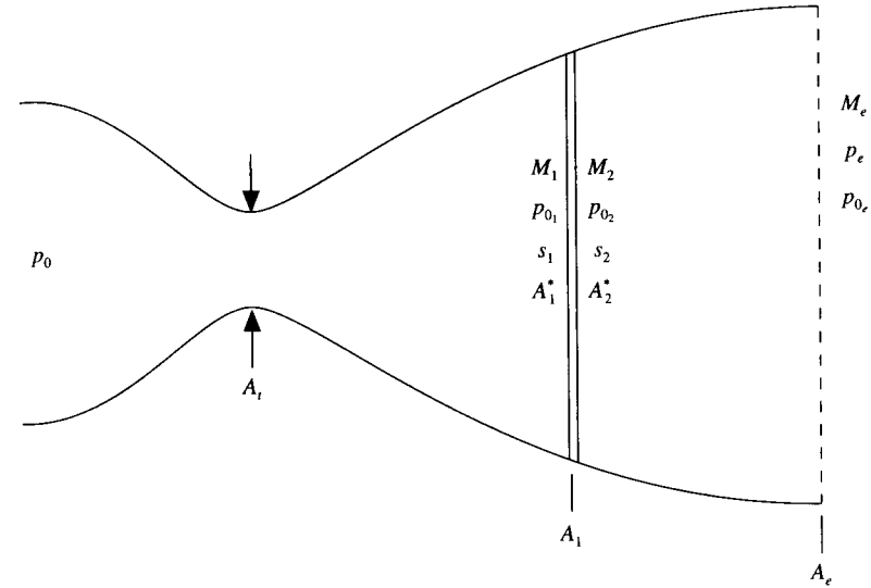
FIG. 7.22 Nomenclature for the normal shock case.
