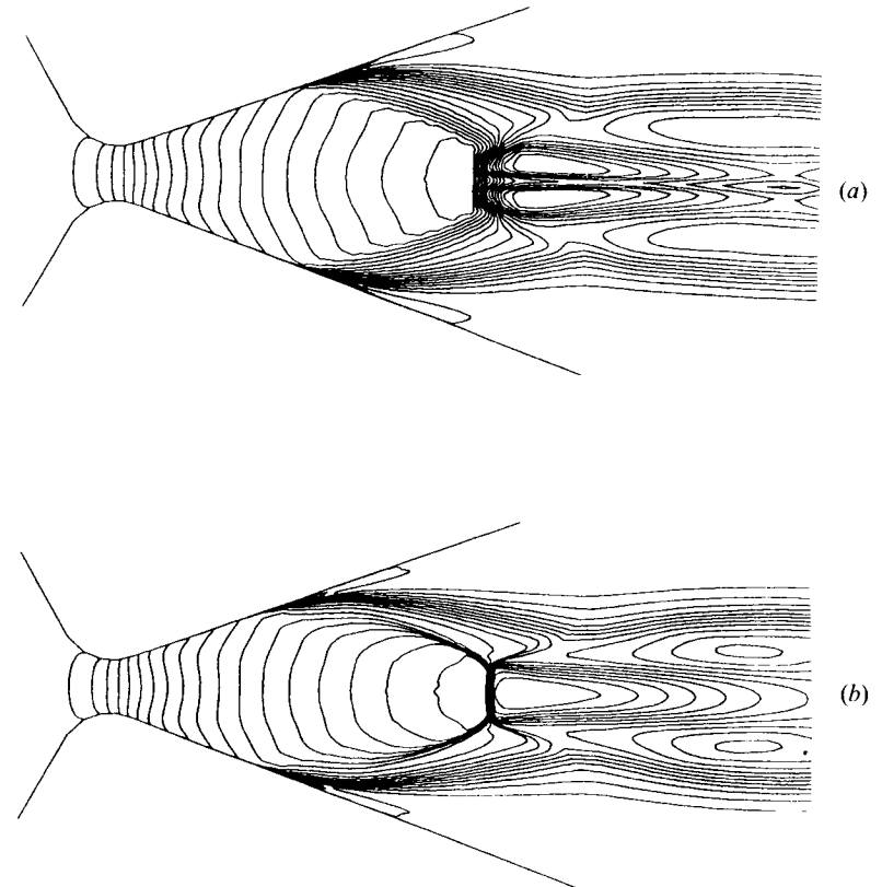
FIG. 12.11 Two-dimensional viscous flow in an overexpanded supersonic nozzle. Mach number contours. Conditions of the flow: p_0/p_e = 50 , A_e/A^* = 7 , \gamma = 1.2 , T_0 = 1800 K. (From Ref. 55. Reprinted with permission from Elsevier Science Publishers, Amsterdam.)
