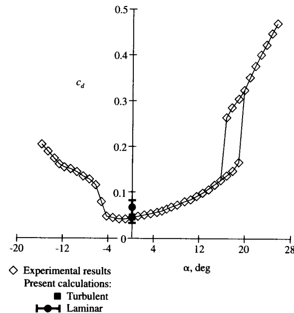
FIG. 1.5 Example of a CFD numerical experiment. Drag coefficient versus angle of attack for a Wortmann airfoil. Re = 100,000 ; M_\infty = 0.5 .
