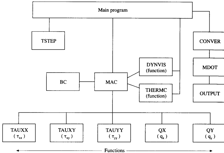
FIG. 10.6 An approach to structuring your code.
