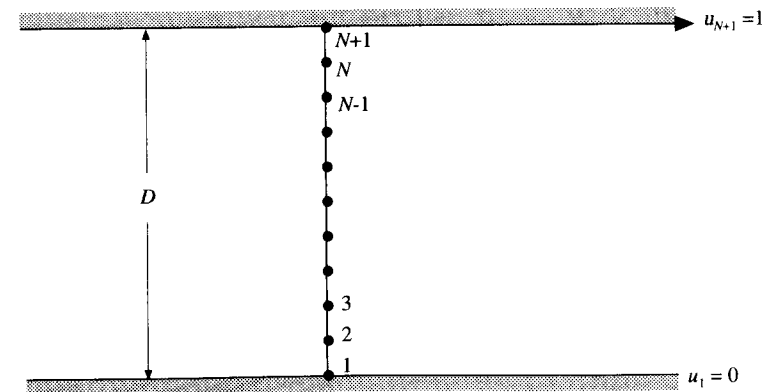
FIG. 9.3 Labeling of points for the grid.
