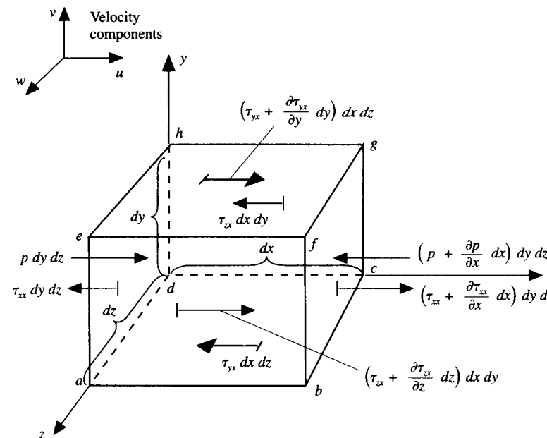
FIG. 2.8 Infinitesimally small, moving fluid element. Only the forces in the x direction are shown. Model used for the derivation of the x component of the momentum equation.
