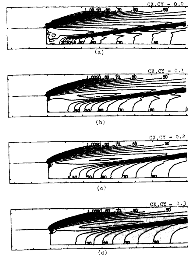
FIG. 6.8 Numerical experiment on the effects of artificial viscosity. Pressure contours calculated with values of the dissipation factors C_x and C_y ranging from 0 to 0.3. The freestream conditions are M_\infty = 4.08 , T_\infty = 1046 K, ratio of specific heats \gamma = 1.31 , and Reynolds number = 849 (based on a step height of 0.51 cm). The wall temperature T_W = 0.2957T_\infty .
