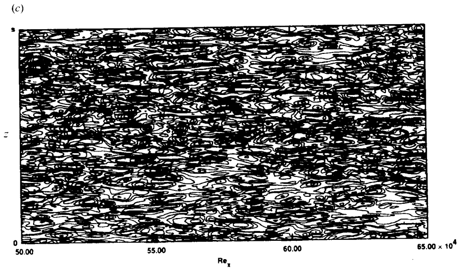
FIG. 12.14 Direct numerical simulation (DNS) of turbulent flow. Vorticity contours looking down at the top of the plate. Parts (a) to (c) correspond to the same time but cover sequentially downstream portions of the plate. (a) Mostly laminar flow; (b) transition from laminar to turbulent flow (transition region); (c) turbulent flow. (From Ref. 57. Copyright © 1991 AIAA. Reprinted with permission.)
