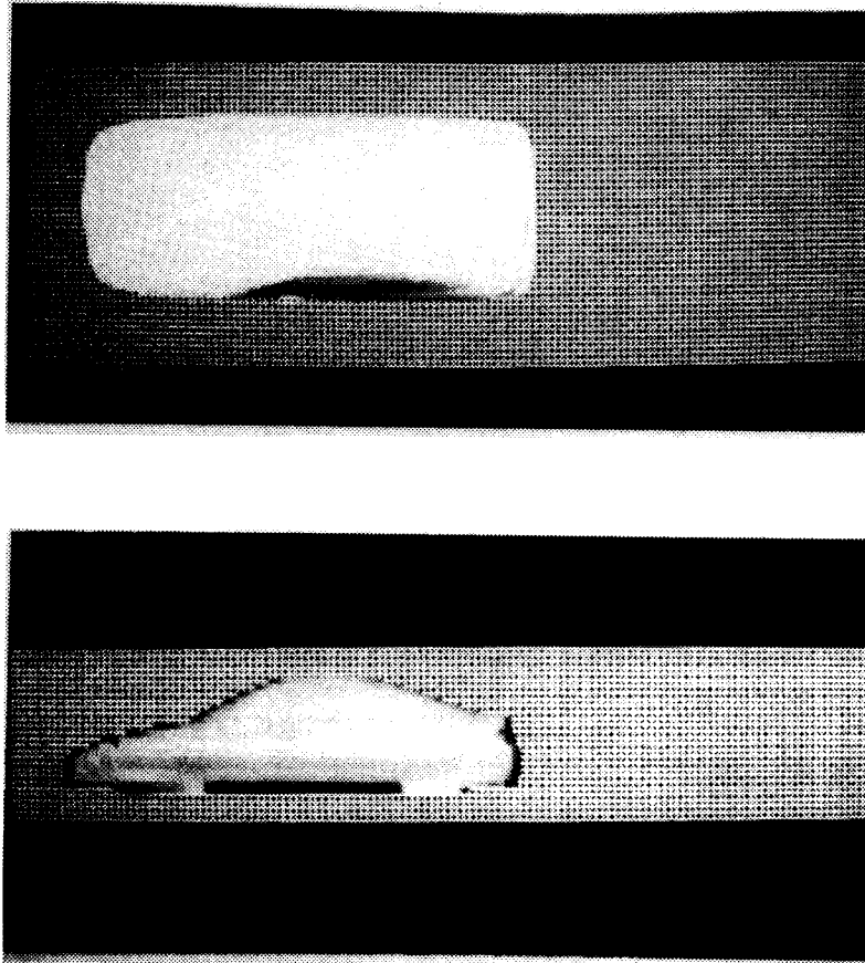
FIG. 1.11 A portion of a rectangular (cartesian) grid wrapped around a car, used for the calculations shown in Fig. 1.10. (From Ref. 59. Reprinted with permission from SAE SP-908, 1992, © 1992 Society of Automotive Engineers, Inc.)
