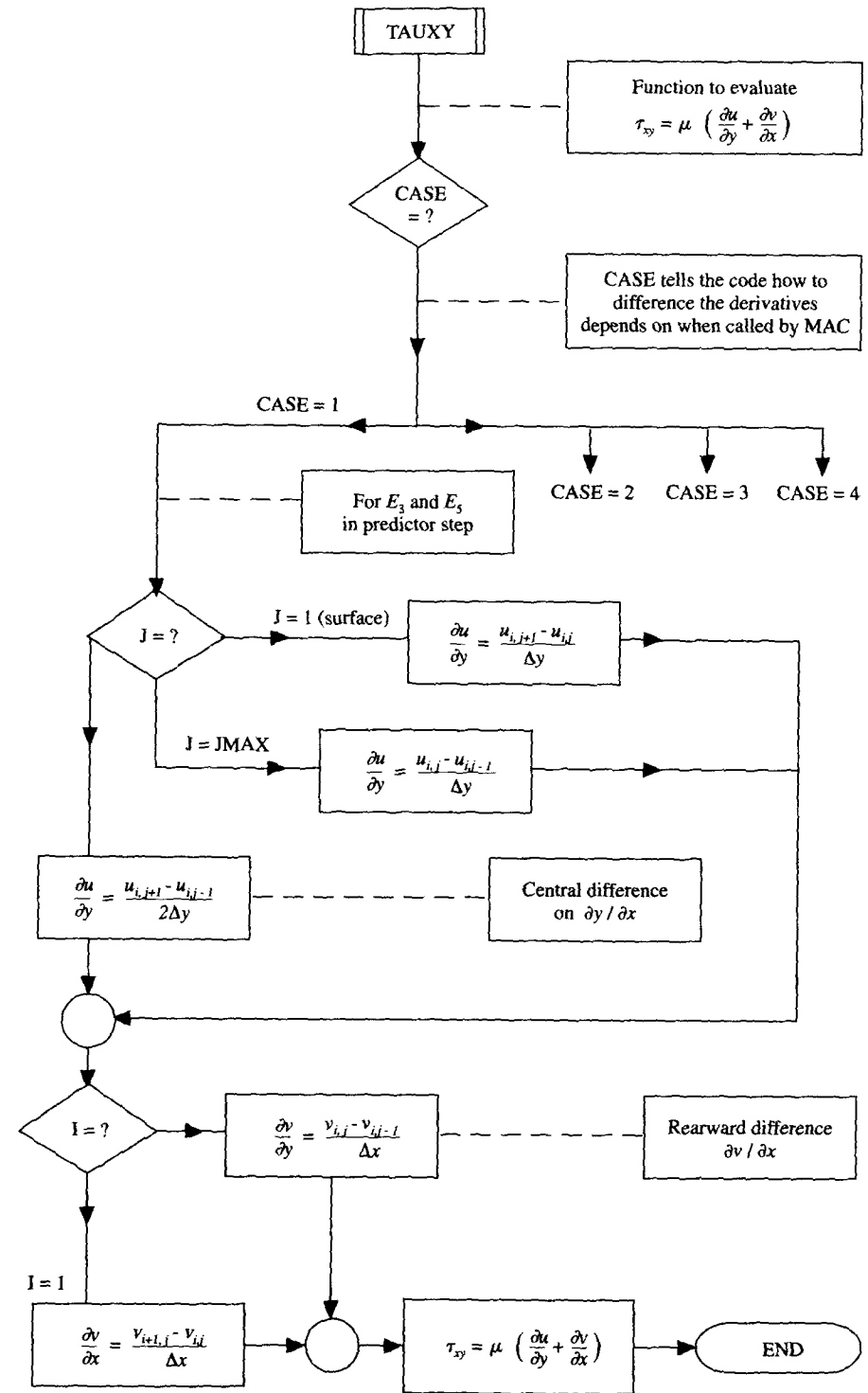
FIG. 10.9 Flowchart for TAUXY function subprogram.
