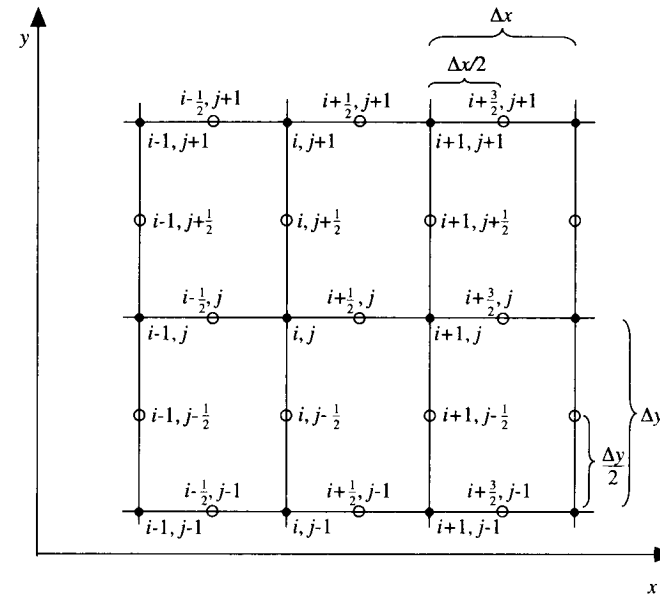
FIG. 6.15 Staggered grid.
