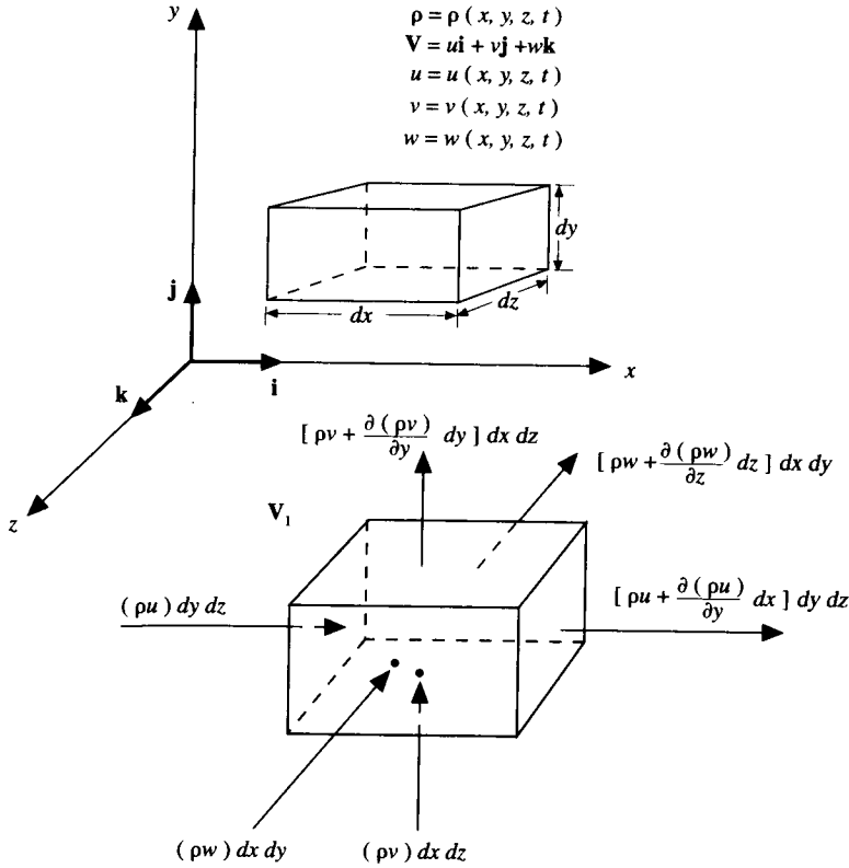
FIG. 2.7 Model of the infinitesimally small element fixed in space and a diagram of the mass fluxes through the various faces of the element—for a derivation of the continuity equation.
