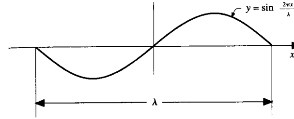
FIG. 4.10 Sine function.
