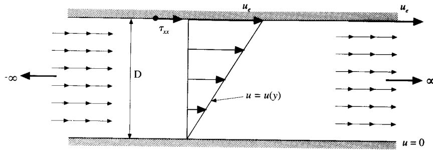
FIG. 9.1 Schematic of Couette flow.
