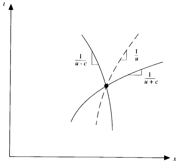
FIG. 11.1 Illustration of the characteristic lines for unsteady, one-dimensional flow.
