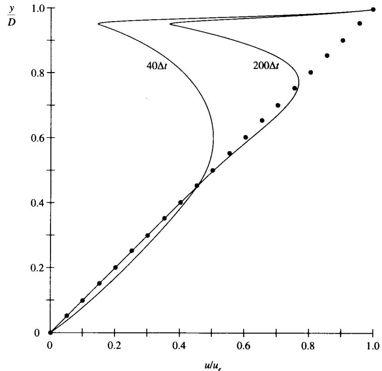
FIG. 9.5 Totally nonphysical transient velocity profiles obtained when E = 4000 ; comparison with exact steady-state results (dark circles).
