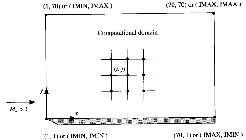
FIG. 10.3 Computational domain.
