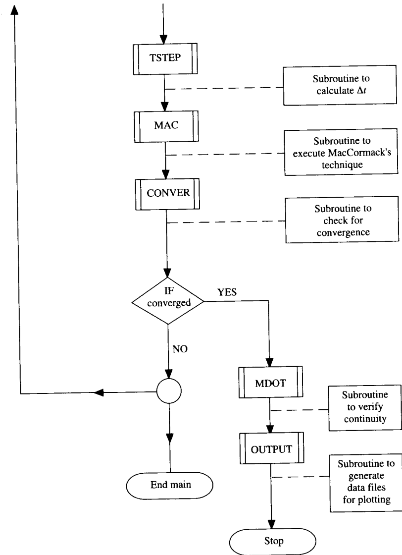
FIG. 10.7 Flowchart for the main program (MAIN).
