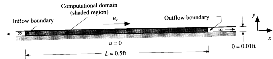
FIG. 9.6 The finite computational domain for the application of the pressure correction method for the solution of the incompressible flow between two plates in relative motion.
